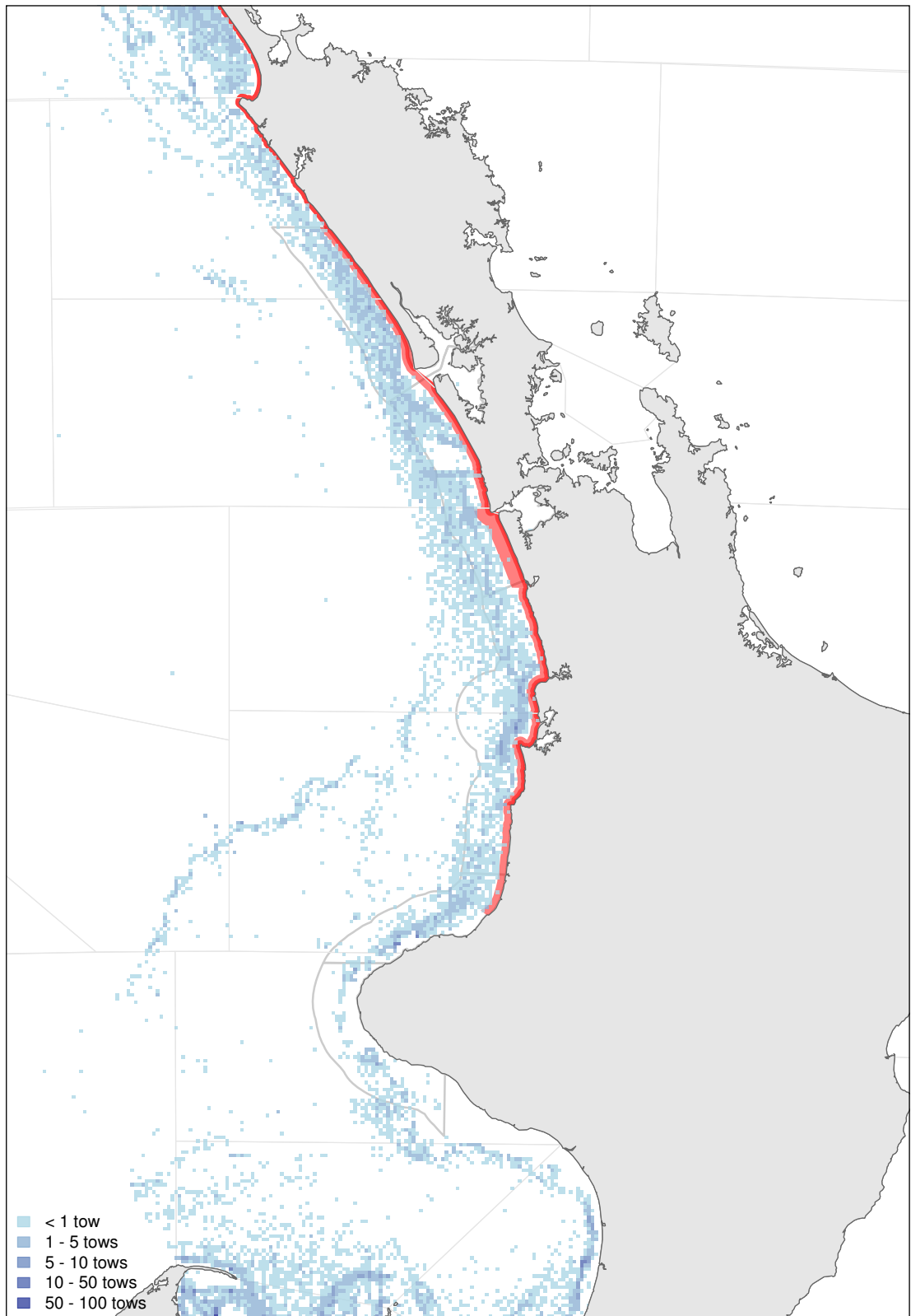
Figure A2.13. Trawl effort from vessels less than 43m long, measured in tows per year, per square nautical mile, for the years 2008 to 2011. The various existing areas closed to trawl fishing are indicated in red. The grey outline marks the extent of the Marine Mammal Sanctuary, including the proposed southern extension.
